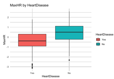
Figure 3: Key numeric predictors by outcome.
